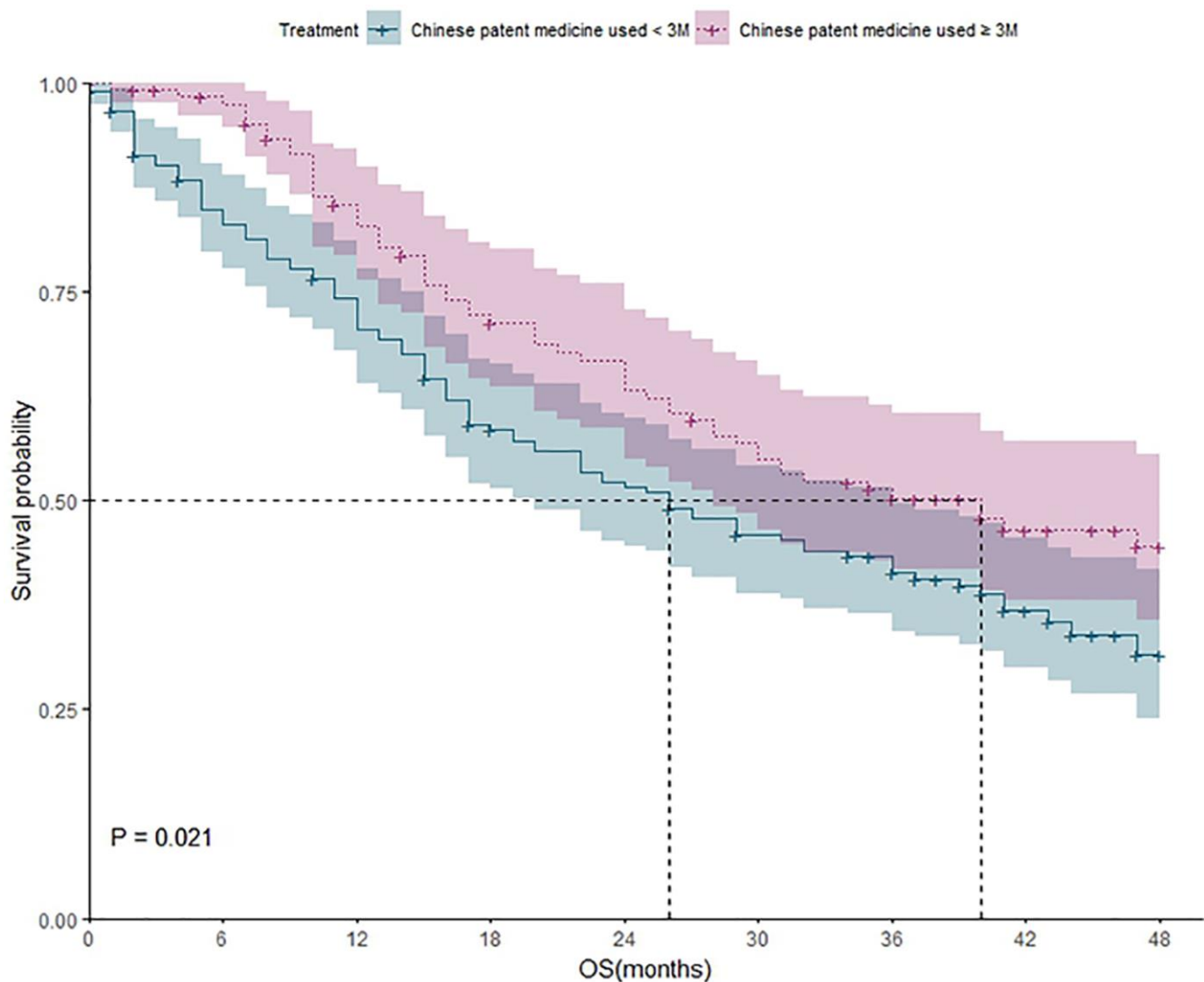
Figure 3. The survival analysis of patients who received CPM for different durations (less than 3 months vs. more than 3 months).
