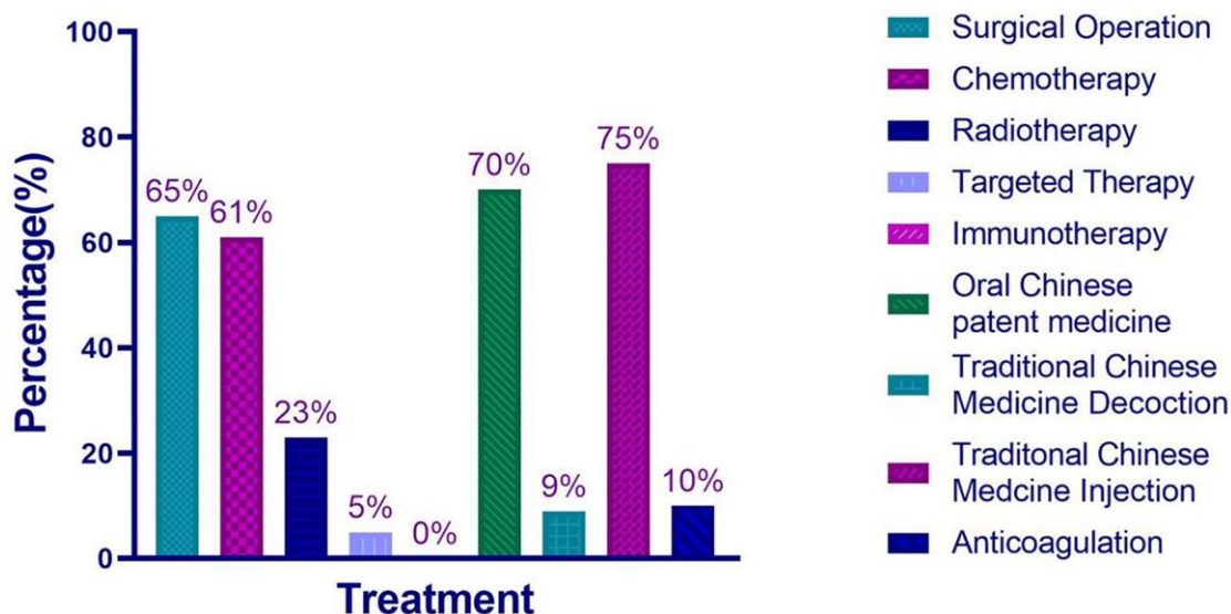
Figure 2. The frequency of each treatment used for 313 patients diagnosed with NSCLC in Sichuan Provincial People's Hospital during 2015–2016.
