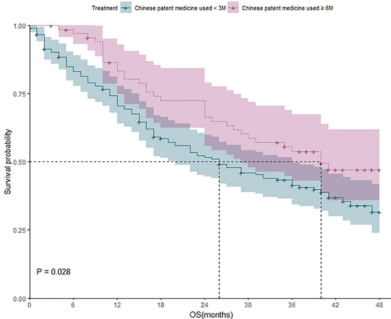
Figure 4. The survival analysis of patients who received CPM for different durations (less than 3 months vs. more than 6 months).
