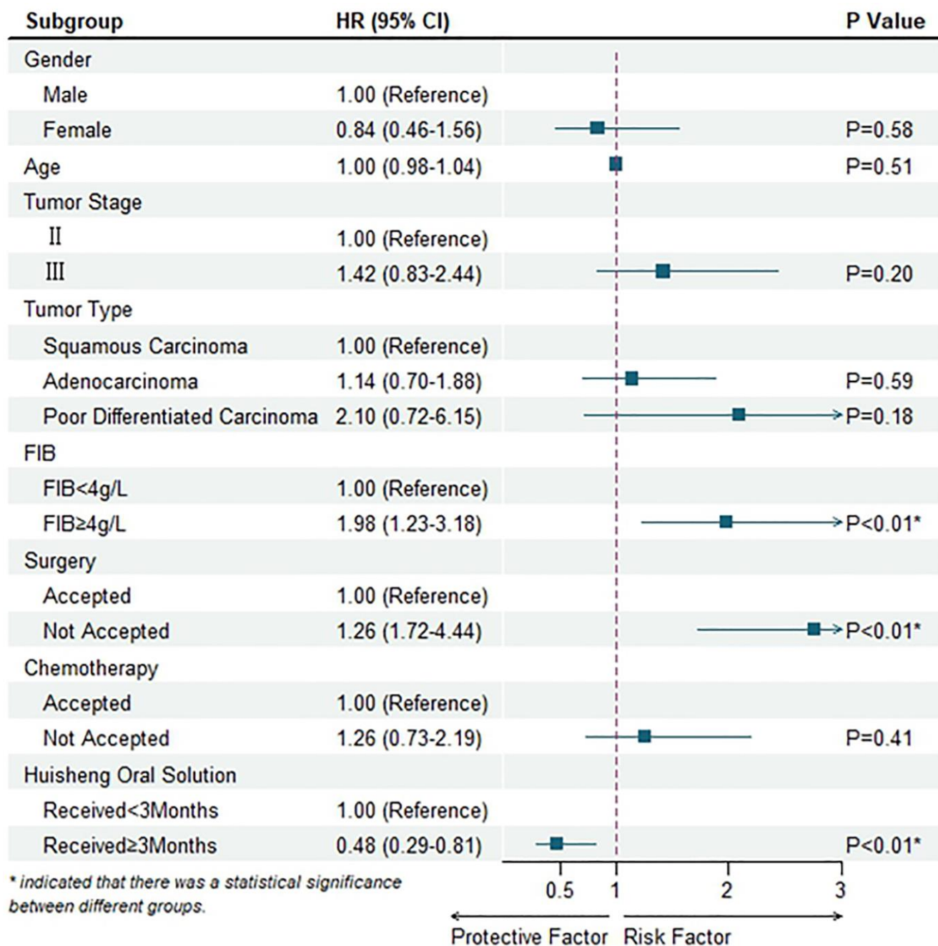
Figure 6. Multivariable Cox regression mode.
