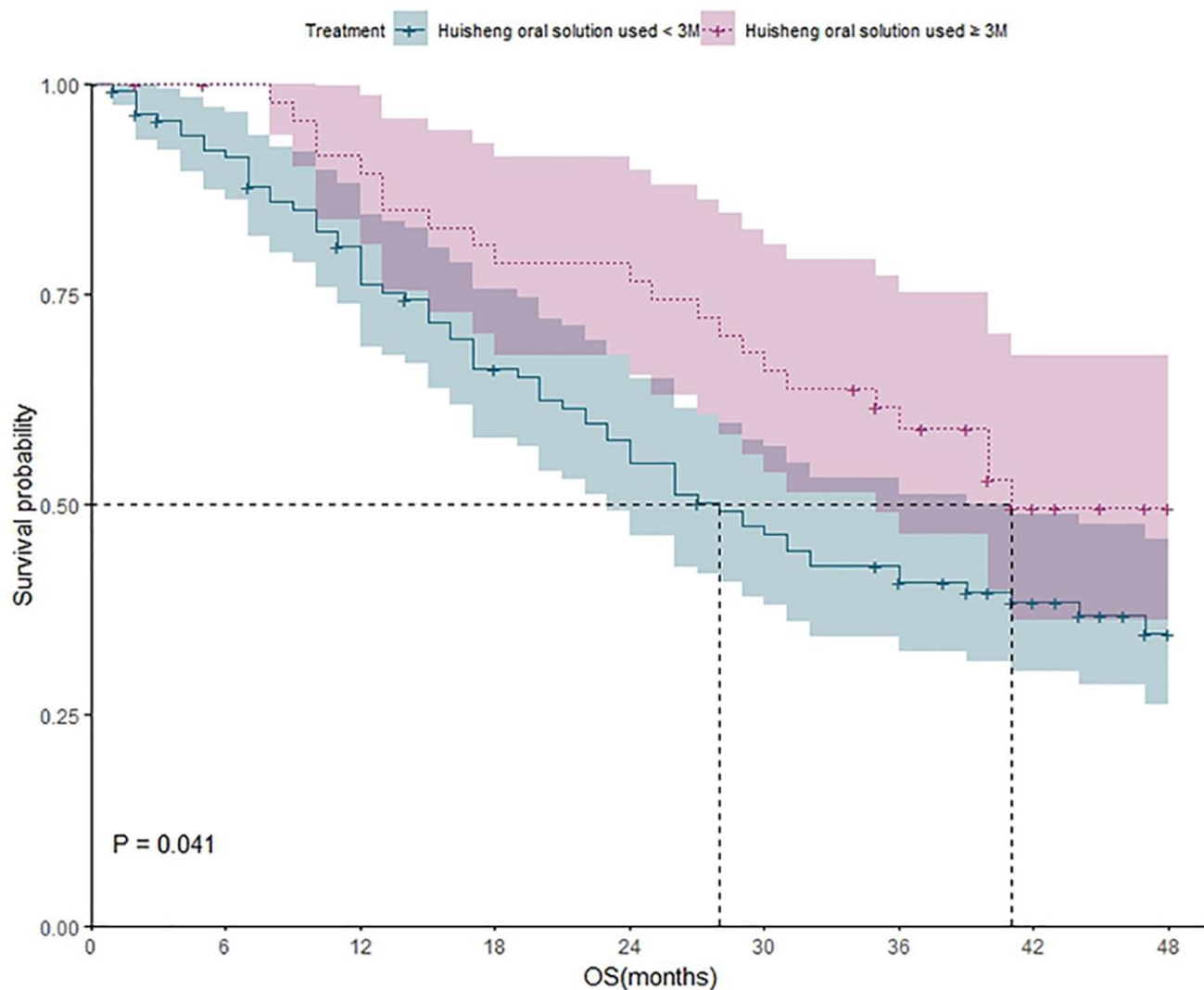
Figure 5. The survival analysis of patients who received HSOS for different durations (less than 3 months vs. more than 3 months).
