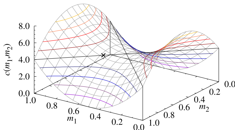
Fig. 1 Surface plot of the injury cost function c(m_1, m_2) of escalated hawk–hawk fights defined by the example given in Eq. (7) with parameter values v = 1 , c_0 = 4 , and \alpha = 16 . \times shows the injury cost at the ESP Eq. (8)
