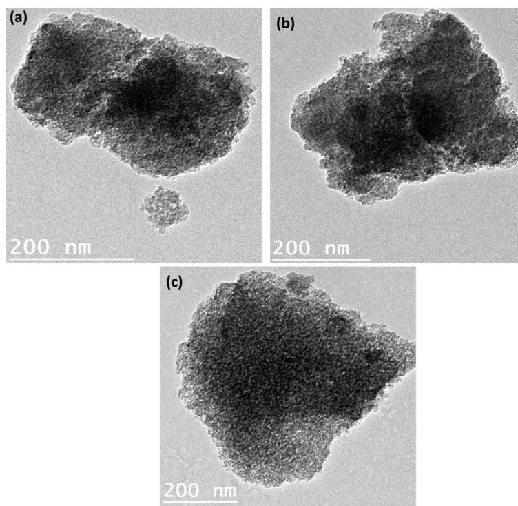
Fig. 1 Particle shape of NIQBD loaded StNPs using TEM where: a StNPs-1, b StNPs-2 and c StNPs-3
