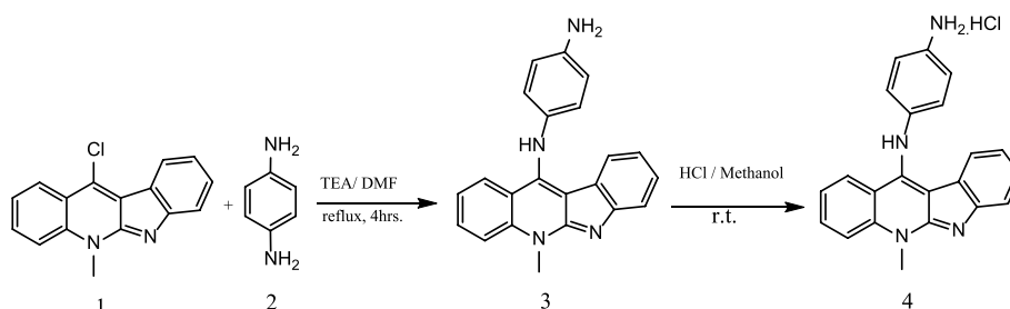
Scheme 2 Synthesis of hydrochloride salt of 4
