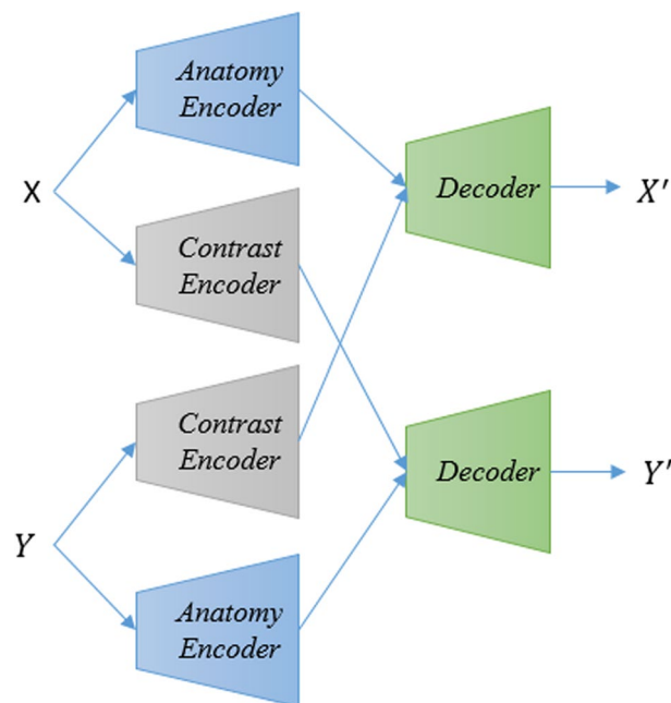
Fig. 7 Disentanglement representation learning diagram
