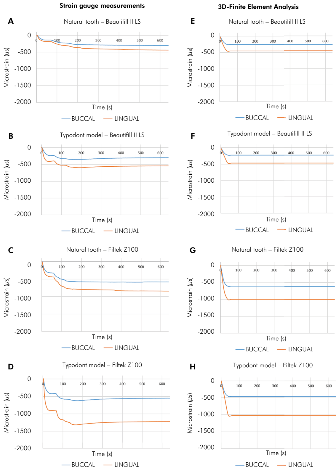
A. Natural tooth - Beautifill II LS; B. Typodont - Beautifill II LS; C. Natural tooth - Filtek Z100; D. Typodont - Filtek Z100. Cuspal strain by 3D finite element analysis: E. Natural tooth - Beautifill II LS; F. Typodont -Beautifill II LS; G. Natural tooth - Filtek Z100; H. Typodont - Filtek Z100.
