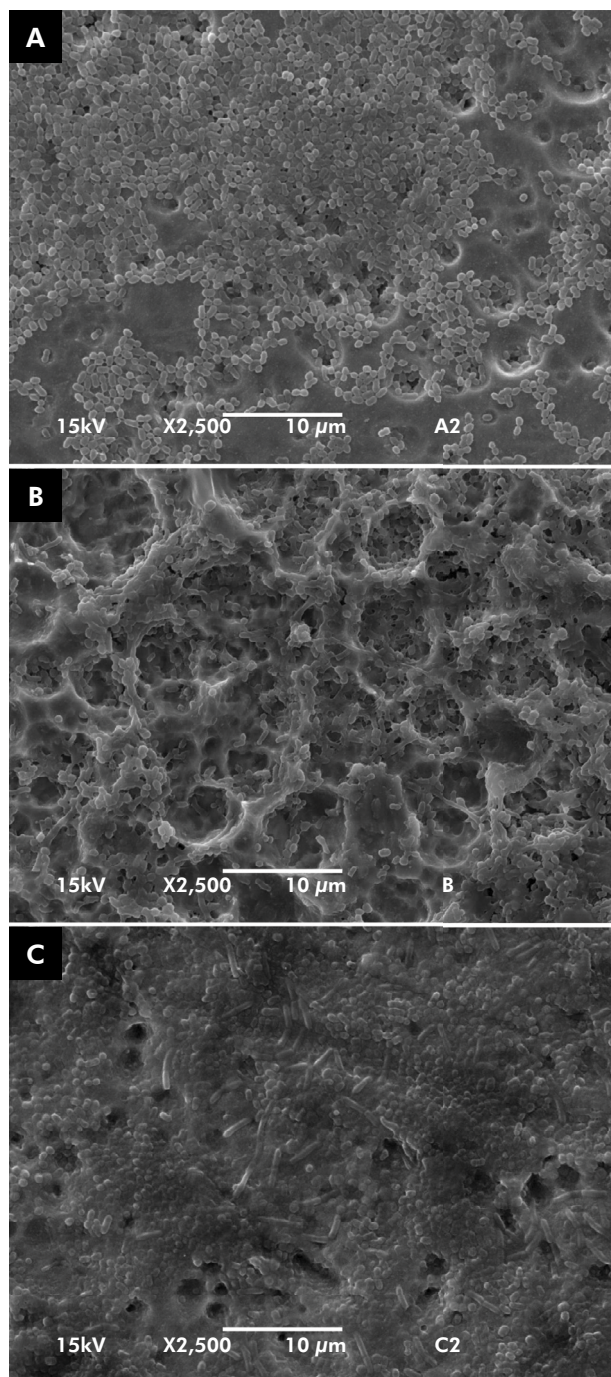
Figure 4. Scanning electron microscopy (2.500x) for Ti-M (1), Ti-Micro (2), and Ti-Nano (3) after in vivo experiments.
