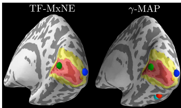
FIGURE 10 | Source localization with non-linear sparse solvers. The left plot shows results from TF-MxNE on raw unfiltered data (due to the built-in temporal smoothing), and the right plot shows results from \gamma -MAP on the same data but filtered below 40 Hz. One can observe the agreement between both methods on the sources in the primary (red) and secondary (yellow) visual cortices delineated by FreeSurfer using an atlas. The \gamma -MAP identifies two additional sources in the right fusiform gyrus along the visual ventral stream. These sources that would not be naturally expected from such simple visual stimuli are weak and peak later in time, which makes them nevertheless plausible.
