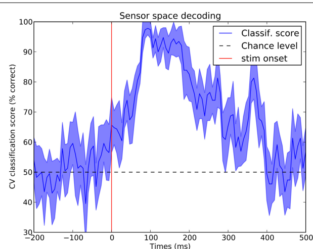
FIGURE 8 | Sensor space decoding. At every time instant, a linear support vector machine (SVM) classifier is used with a cross-validation loop to test if one can distinguish data following a stimulus in the left ear or in the left visual field. One can observe that the two conditions start to be significantly differentiated as early as 50 ms and maximally at 100 ms which corresponds to the peak of the primary auditory response. Such a statistical procedure is a quick and easy way to see in which time window the effect of interest occurs.
