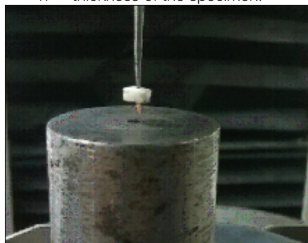
[Table/Fig-1]: Specimen mounted on universal testing machine [Table/Fig-2]: Extrusion of filling material
