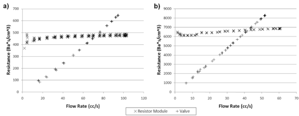
Fig 8. Resistance v.s. Flow Rate for Resistor Module with Theoretical Resistance of a) 500 Ba*s/cm 3 , b) 6700 Ba*s/cm 3 , and a Partially Closed Ball Valve
