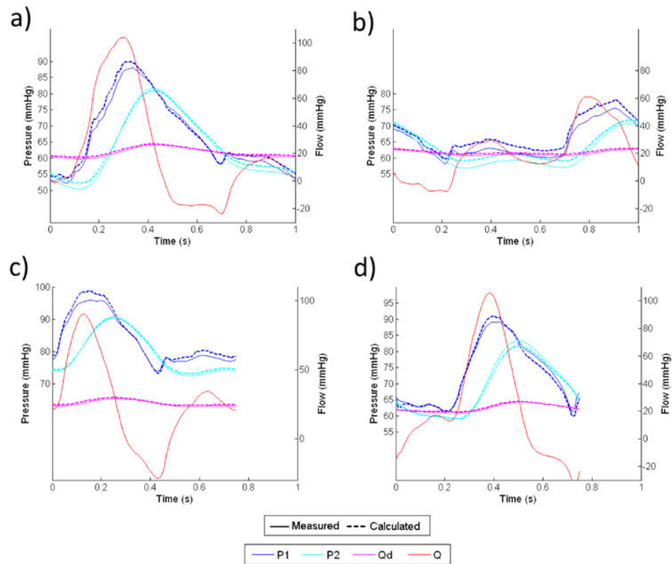
Fig 9. Comparisons Between Measured(solid lines) and Calculated(dashed lines) Pressure & Flow Waveforms for the Thoracic-Aortic Impedance Module Under Four Different Flow Conditions: a) Flow Condition 1, b) Flow Condition 2, c) Flow Condition 3, and d) Flow Condition 4
