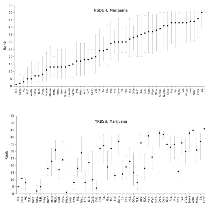
Figure 3. States' simulated ranks for adolescent (aged 14–17 y) marijuana use as reported in the National Survey on Drug Use and Health (NSDUH) or Youth Risk Behavior Surveillance System (YRBSS), 2011–2015. Past-month marijuana use was defined as using marijuana at least once in the previous 30 days. YRBSS data were collected in 2011, 2013, and 2015; District of Columbia, Minnesota, Oregon, and Washington were excluded from YRBSS because they either chose not to participate or did not achieve adequate response rates. Data on marijuana use in YRBSS were not available for Hawaii. States are ordered by median rank in NSDUH across 100,000 simulations. Error bars indicate 95% confidence intervals.
