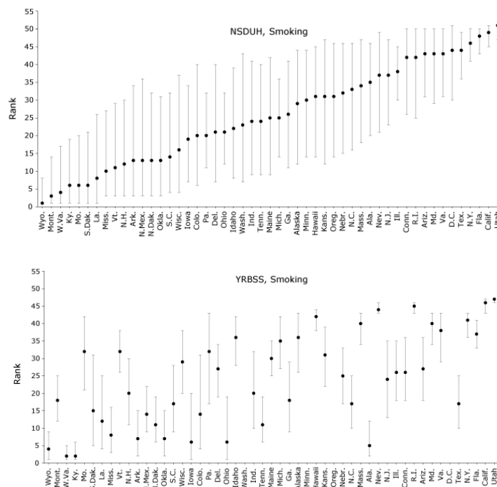
Figure 1. States' simulated ranks for adolescent (aged 14–17 y) cigarette smoking as reported in the National Survey on Drug Use and Health (NSDUH) or Youth Risk Behavior Surveillance System (YRBSS), 2011–2015. YRBSS data were collected in 2011, 2013, and 2015; District of Columbia, Minnesota, Oregon, and Washington were excluded from YRBSS because they either chose not to participate or did not achieve adequate response rates. Past-month cigarette smoking was defined as smoking at least 1 cigarette in the previous 30 days. States are ordered by median rank in NSDUH across 100,000 simulations. Error bars indicate 95% confidence intervals.
