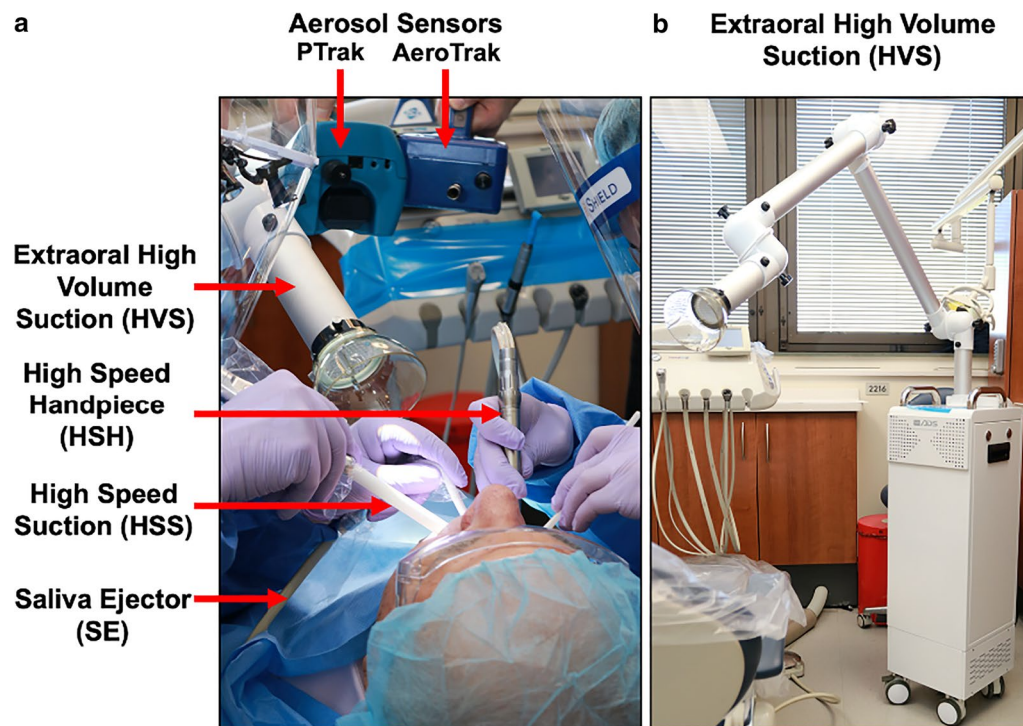
Fig. 1 Experimental setup for the dental procedures and aerosol measurements. a Locations of the different suction systems including saliva ejector (SE), high speed suction (HSS) and extraoral high volume suction (HVS). Locations of the aerosol meters during data acquisition. b The HVS device use for the experiment
