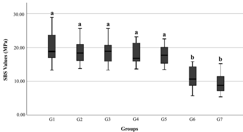
Fig. 6 The shear bond strength test in seven groups. Different lower-case letters indicate the significant statistical difference ( p < 0.05 )
