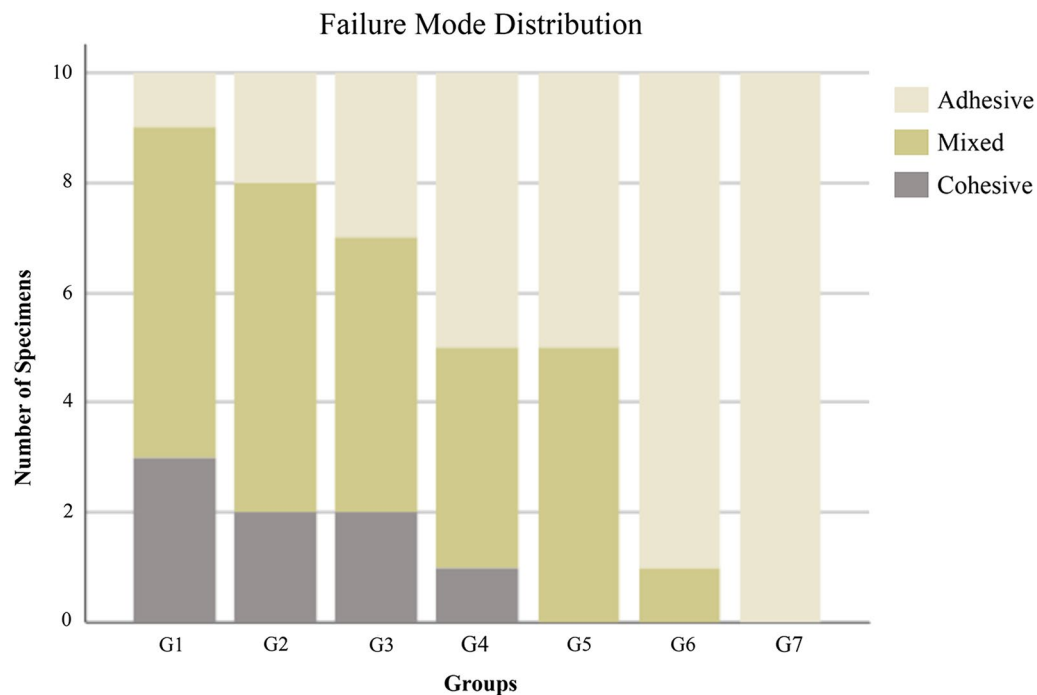
Fig. 7 Distribution of adhesive failure types among seven groups
