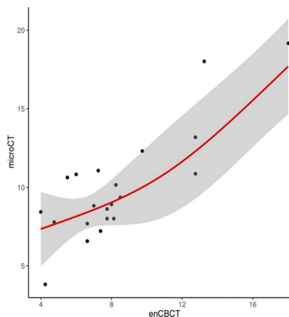
Fig. 8 Risk-adjusted, restricted cubic splines with 4 knots of crack depths measured by contrast-enhanced CBCT and crack depths measured by micro-CT. The X axis shows the crack depths measured using contrast-enhanced CBCT; the Y axis shows the crack depths measured using micro-CT. Red line represents crack depths measured using micro-CT; Grey area represents a 95% confident interval. The root mean square error (RMSE) was 1.813, R^2 was 0.724, P=0.000 . Micro-CT: micro-computed tomography; contrast-enhanced CBCT: contrast-enhanced cone beam computed tomography
