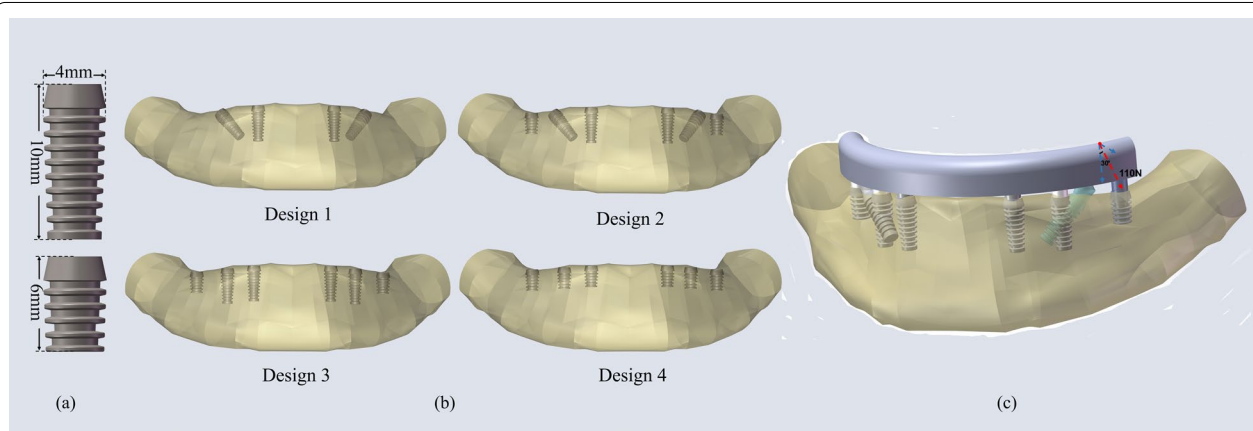
Fig. 2 a two specifications of implants, b four implants restoration designs, c 110N oblique load applied on the framework at the left second premolar site
