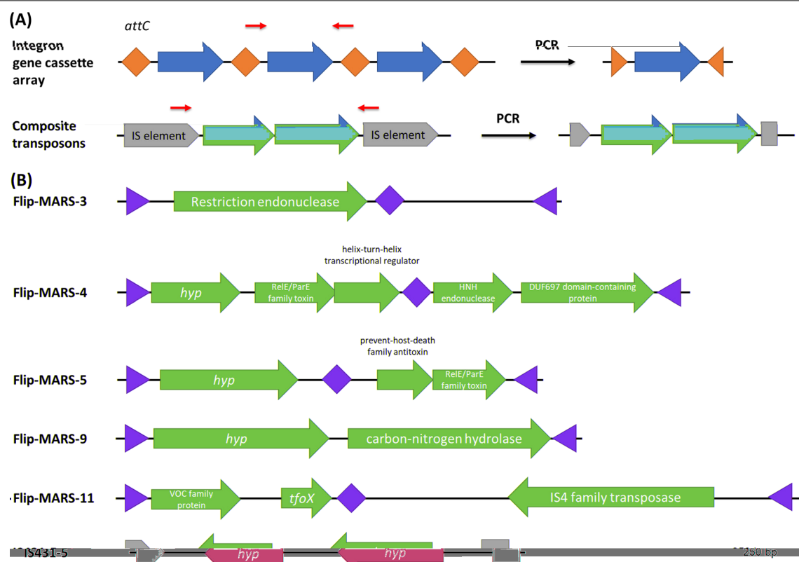
Fig. 2 The predicted structures of the genetic context of integron GC and composite transposon samples detected from the oral metagenome. A The general structures of integron and composite transposons B The integron GC and composite transposons identified from the oral metagenome by IPCR. Genes associated with both types of MGEs were amplified from the DNA fragment (blue open arrows) located in between two DNA repeats which are attC recombination site of integrons (orange diamond shapes) and IS elements of composite transposons (grey open arrows)
