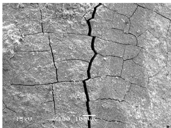
Fig. 12 The crack pattern in instrumented group
