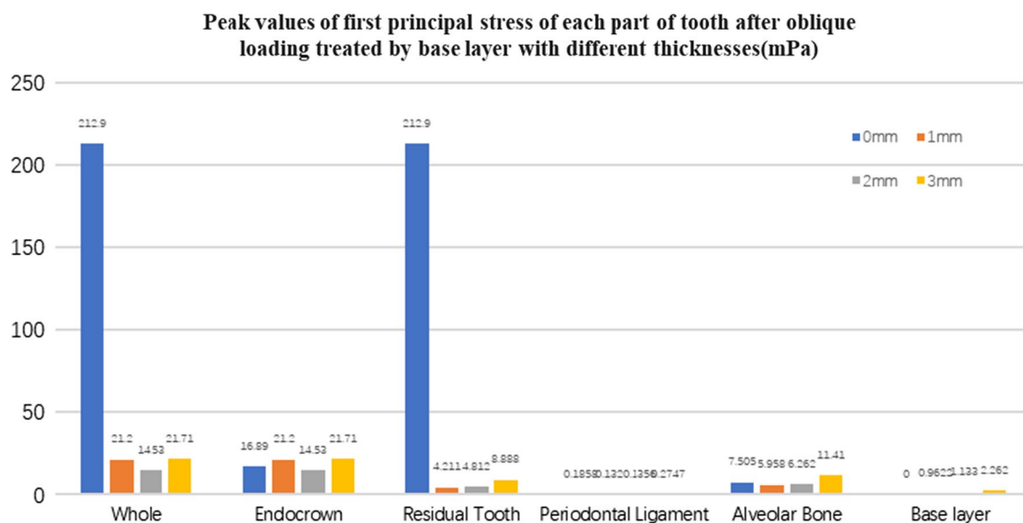
Fig. 24 The first stress peak value (mPa) of each part of tooth body treated with different thickness of base materials (fluid resin) under oblique loading
