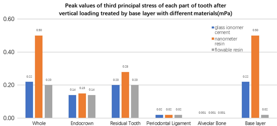
Fig. 30 The third stress peak (mPa) of each part of the tooth body treated with different base materials under vertical loading
