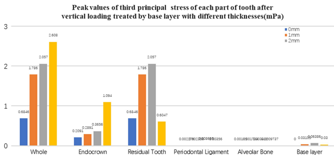
Fig. 14 The third principal stress peak (mPa) of each part of the tooth body treated with different thicknesses of base material (fluid resin) under vertical loading
