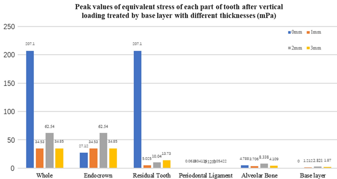
Fig. 11 The peak values of equivalent stress (mPa) of each part of the tooth body treated with different thicknesses of base material (fluid resin) under vertical loading
