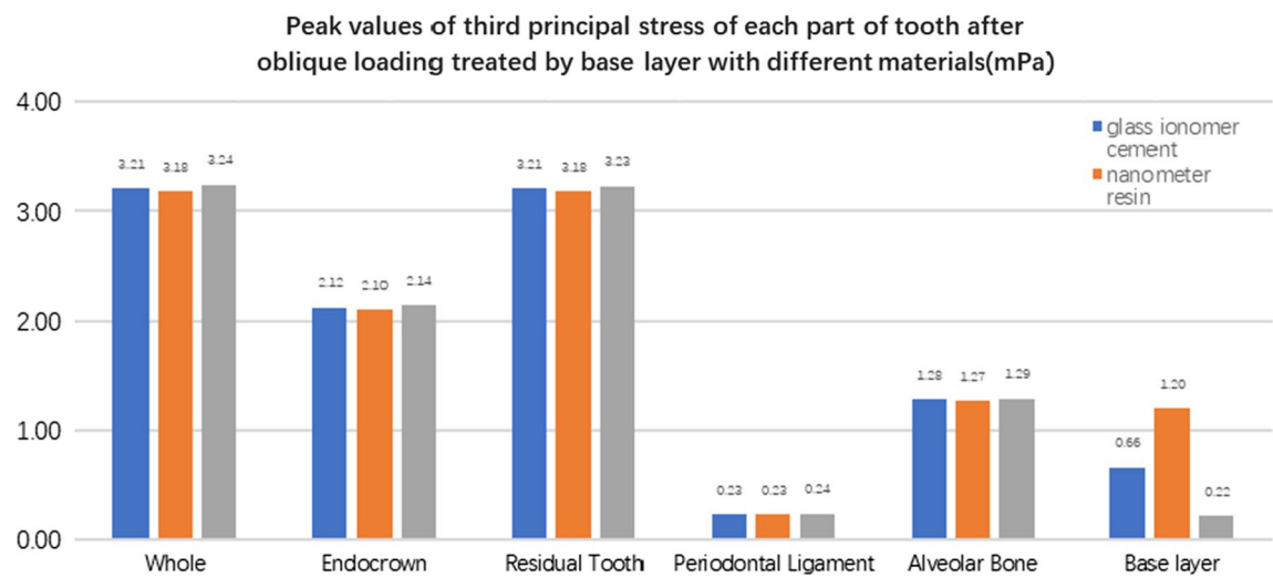
Fig. 34 The third stress peak (mPa) of each part of the tooth body treated with different bedding materials under oblique loading
