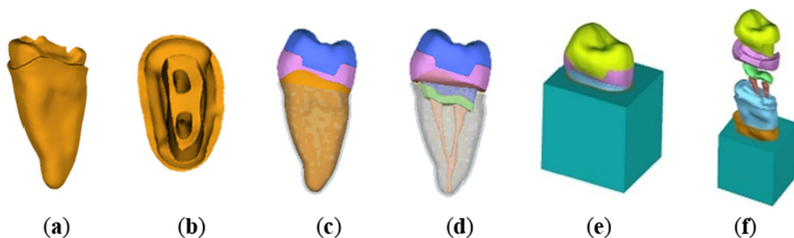
Fig. 1 Design of abutment components based on Geomagic software
