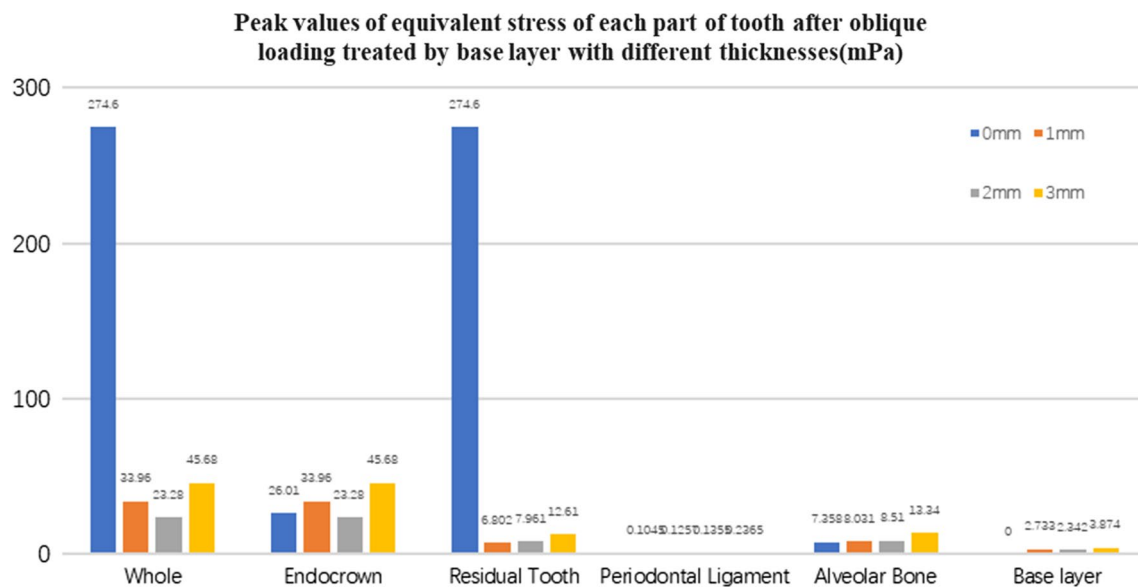
Fig. 23 The equivalent stress peak value (mPa) of each part of tooth body treated with different thickness of base materials (fluid resin) under oblique loading
