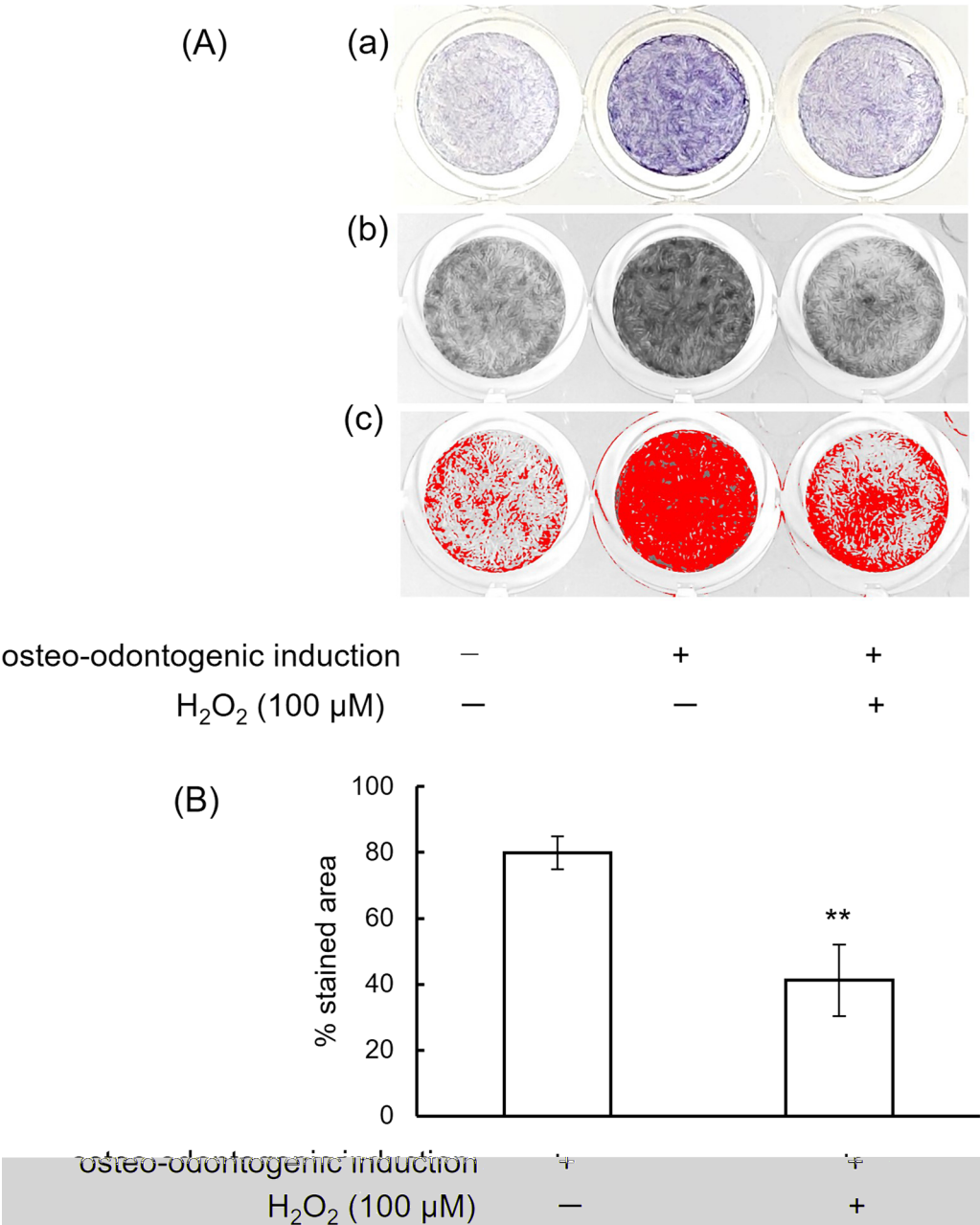
Fig. 2 H 2 O 2 attenuates ALP activity of hDPCs. A(a) A macroscopic view of wells showing hDPCs cultured in growth medium, hDPCs cultured in osteo-odontogenic medium, and hDPCs treated with 100 μM H 2 O 2 in osteo-odontogenic medium. (b) A(a) panels were converted to RGB stack, and “blue slices” were picked up. (c) The thresholds of the images of A(b) were adjusted, and a limited threshold area is highlighted in red. B The stained area was quantified using Image J software on digitized photomicrographs ( A(c) ) captured by a Windows-based computer. Values are expressed as means ± SD of three independent experiments. ** P < 0.01, Student’s t -test
