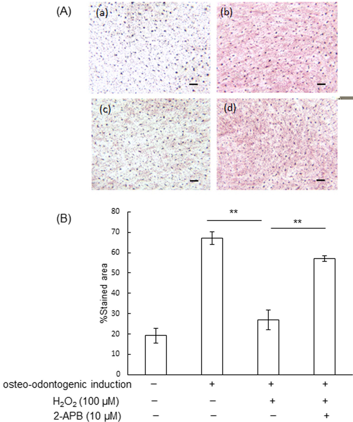
Fig. 4 Assessment of hDPC calcification with Alizarin red staining. A Panels show hDPCs cultured in growth medium (a), hDPCs cultured in osteo-odontogenic medium (b), hDPCs treated with 100 μM H 2 O 2 in osteo-odontogenic medium (c) and hDPCs treated with 10 μM 2-APB before the addition of 100 μM H 2 O 2 in osteo-odontogenic medium (d). Bars: 100 μm. B The amount of calcium was quantified using Image J software on digitized photomicrographs captured by a Windows-based computer. Data are presented as means ± SD of three independent experiments. ** P < 0.01, one-way ANOVA with Tukey's test
