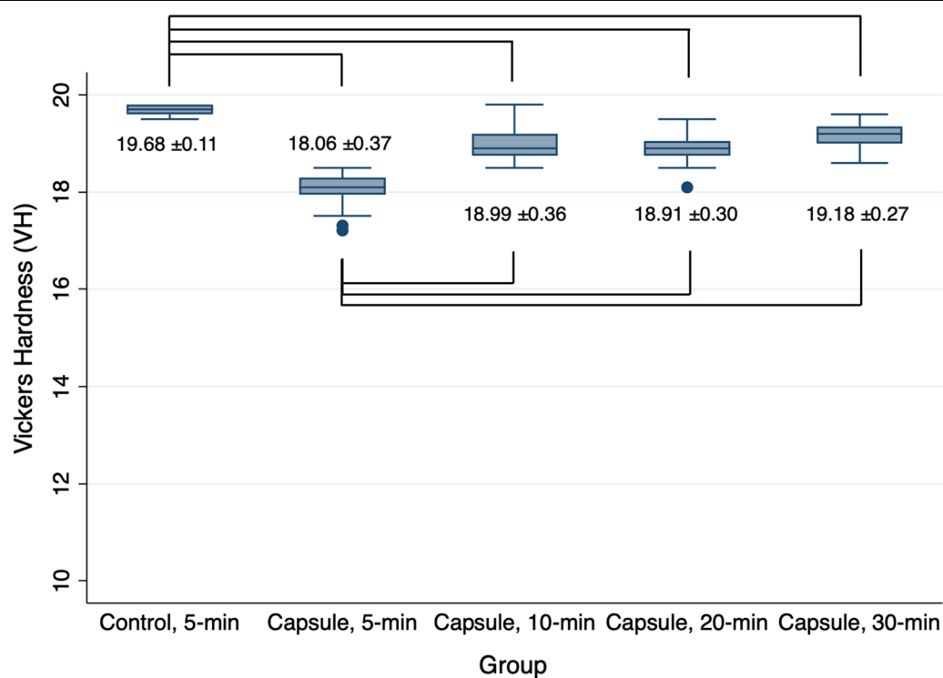
Fig. 5 Vickers hardness (VH) of 3D-printed denture base resin discs subjected to different post-polymerization time (PPT) protocols: 5-min, 10-min, 20-min, and 30-min. Control: 3D-printed denture base resin discs without microcapsules; Capsule: 3D-printed denture base resin discs with 5 wt% phytoncide-filled microcapsules. Significant differences between the groups are marked with black lines ( P < 0.05 )
