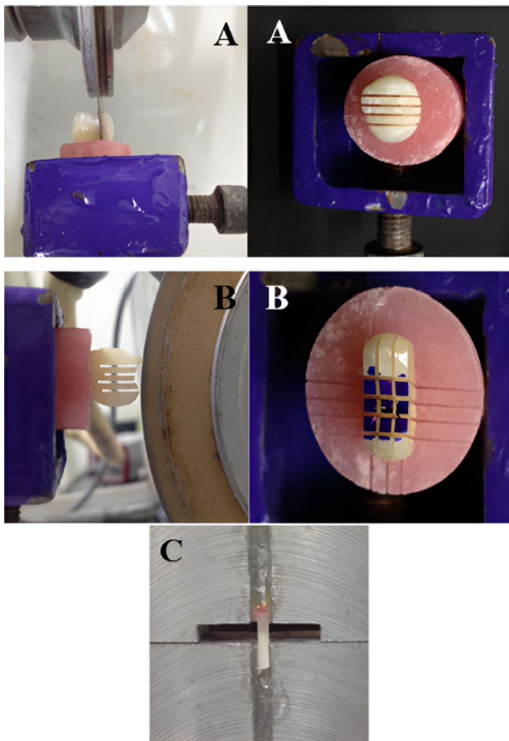
Fig. 7 The specimen preparation for \mu TBS testing A The specimen was sectioned in occluso-lingual direction B The specimen was rotated 90^\circ and cut was made perpendicular to occlusal surface to gain 1 \pm 0.1 \text{ mm}^2 rectangular beams C Beam glued to Geraldini's jig
