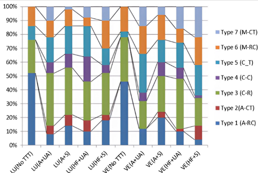
Fig. 8 Failure patterns in percentages among tested groups
