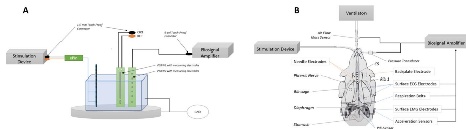
Fig. 2 In vitro test setup A used for the analysis of stimulation intensities with directed as compared to omnidirectional electrodes and animal trial setup B with dedicated stimulation and measurement equipment
