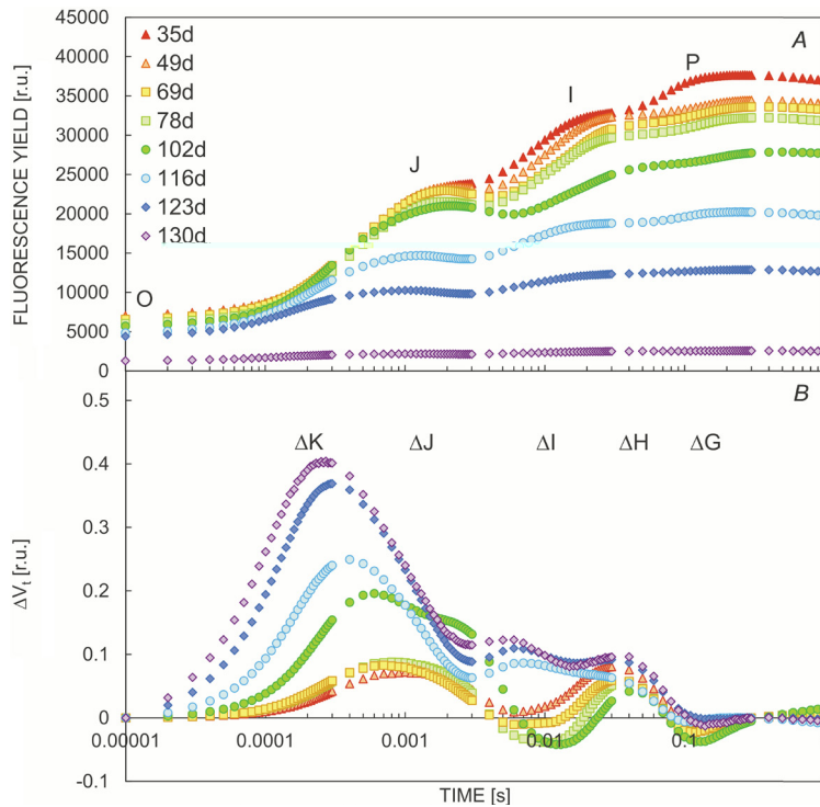
Fig. 2. Chlorophyll a fluorescence induction curve of Vitis vinifera L. during aging period of growing season (A) and the effect of aging of PSII on the relative variable fluorescence [ \Delta V_t = (F_t - F_0)/F_v - V_{t35d} ] of studied leaves (B). For \Delta V_t analysis, the fluorescence of leaves on day 35 of the measurements was used as a reference and equalled 0. Values are means ( n = 30 ).
