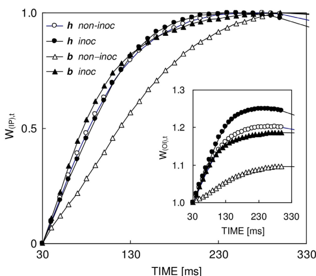
Fig. 8. The average Chl a fluorescence transients, depicted in Fig. 2, of dark-adapted needles of Pinus halepensis ('h', circles) and Pinus brutia ('b', triangles) trees grown in a gypsum quarry (in Cyprus), without (open markers) or with inoculation with a commercial mixture of ectomycorrhiza (closed markers), are expressed and plotted on a linear time scale in the range of the IP-phase as W_{(IP),t} = (F_t - F_I)/(F_P - F_I) = f(t) in the main plot and W_{(OI),t} = (F_t - F_0)/(F_I - F_0) = f(t) in the insert.
