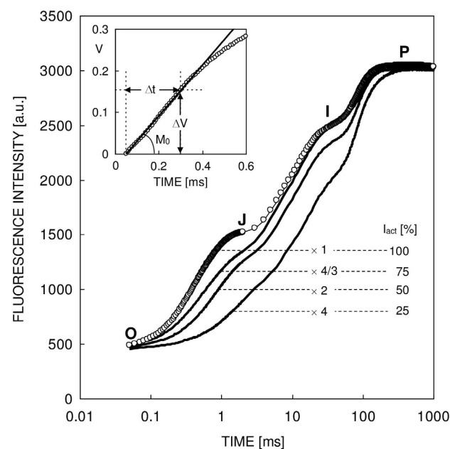
Fig. 1. A typical Chl a fluorescence rise kinetics OJIP ( open circles ), exhibited upon illumination of a dark-adapted photosynthetic sample (here a pea leaf) by strong red light [3,000 \mu mol(photon) m^{-2} s^{-1} ; peak at 650 nm] and measured with the PEA -fluorimeter, plotted on a logarithmic time scale; the steps O (at 50 \mu s), J (at 2 ms), I (at 30 ms), and P (peak) are marked. Transients obtained with lower actinic light intensities, I_{act} (indicated as percentages of the highest intensity used) are also depicted ( lines , no markers). In order to facilitate comparison, the obtained data with I_{act} : 100, 75, 50, and 25% were multiplied by 1, 4/3, 2, and 4, respectively. The insert depicts the transient obtained with the maximal I_{act} , expressed as relative variable fluorescence V_t = (F_t - F_0)/(F_M - F_0) = f(t) , plotted on a linear time scale from 50 \mu s to 0.6 ms, demonstrating how the initial slope is calculated: M_0 = (\Delta V/\Delta t)_0 = (V_{300\mu s})/(0.25 \text{ ms}) .
