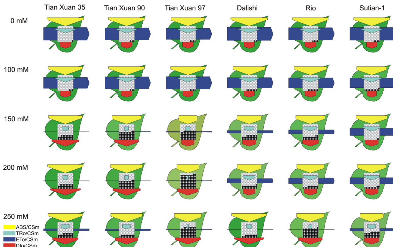
Fig. 5. Leaf pipeline model showing the proportion of phenomenological energy fluxes within a leaf calculated per excited cross section ( CS_m ). Models are drawn with Biolzyzer software. The value of each parameter can be seen in relative changes in width of each arrow (see the color legend). Active RCs are shown as open circles and inactive RCs are closed circles . ABS/CS_m – absorption per excited cross section; DI_o/CS_m – effective dissipation of energy per excited cross section; ET_o/CS_m – electron transport flux from reduced Q_A to Q_B per excited cross section; TR_o/CS_m – maximal trapping rate of absorbed photons per excited cross section.
