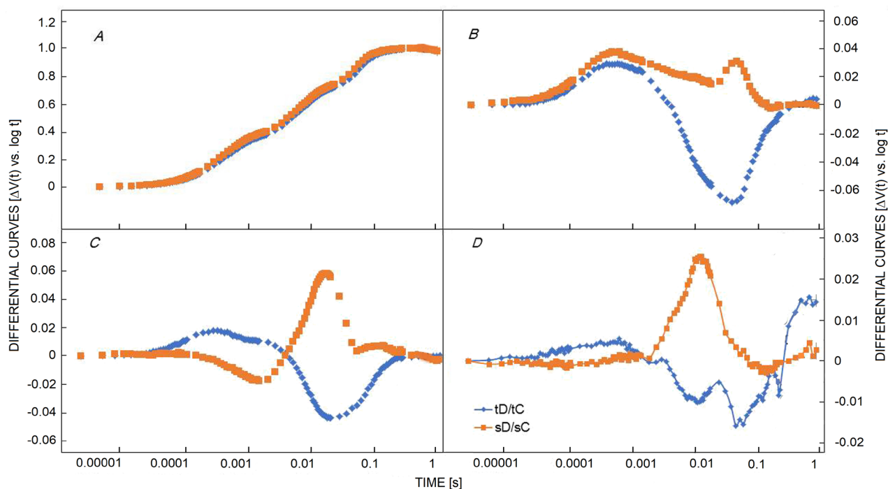
Fig. 2. Double normalized original OJIP transients (A) and differential ( i.e. , \Delta V(t) = V_{(t)DS} - V_{(t)C} ) chlorophyll fluorescence induction curves (B–D) of dark-adapted leaves of the drought tolerant maize accession Zea 1006 and the drought sensitive accession Zea 612 under drought stress as compared to the controls, after drought exposure for 3 (A), 11 (B), 14 (C), and 17 d (D). Blue curves are for Zea 1006 and red curves are for Zea 612.
