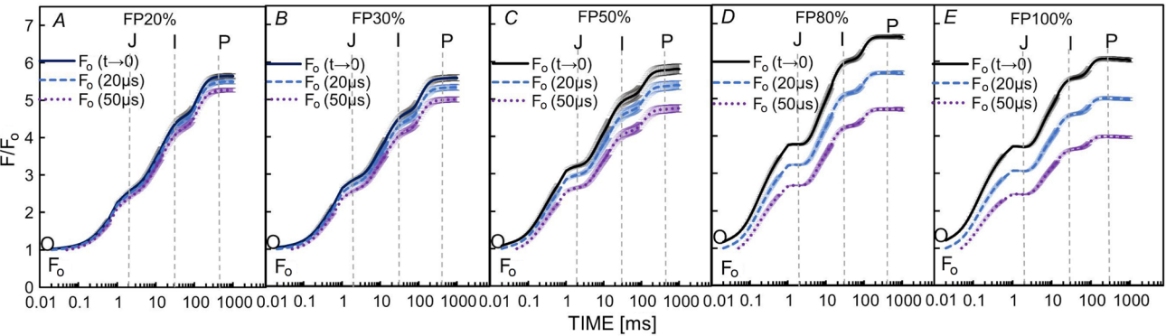
Fig. 3. Chl a fluorescence induction (OJIP) curves measured under different light intensities and normalized to F_o (extrapolated) at t = 0 ( F_{t \rightarrow 0} ), F_{20\mu\text{s}} , and F_{50\mu\text{s}} . Data obtained with FluorPen (FP) (excitation light, \lambda = 470 \text{ nm} ) on 20-min dark-adapted intact leaves of wild type Arabidopsis thaliana , under different light intensities [where 100% light intensity is 3,120 \pm 87 \mu\text{mol}(\text{photons}) \text{ m}^{-2} \text{ s}^{-1} ; see Table 1 ], the curves are averages of 15 replicates \pm SE.
