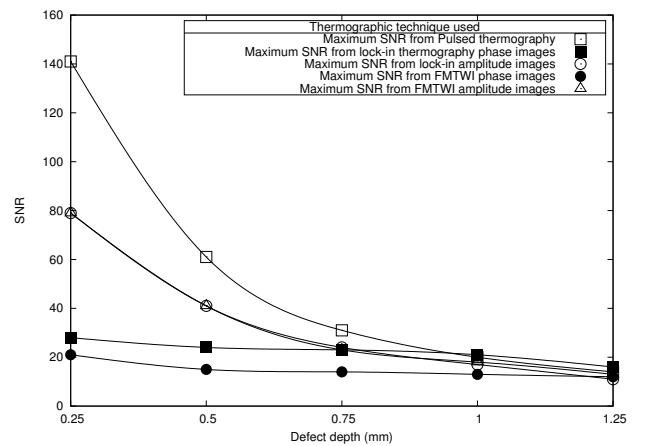
Figure 10: Plot of maximum SNR as a function of defect depth, as in Table 6
