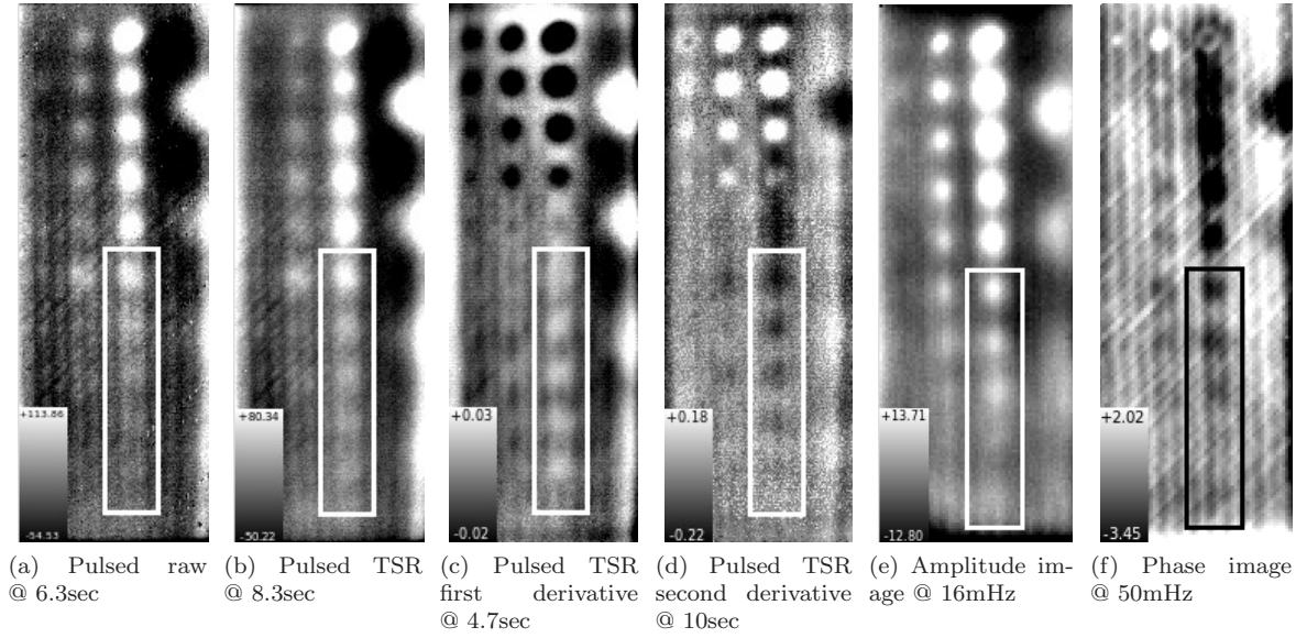
Figure 12: Comparison with TSR
