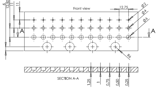
Figure 1: Test piece dimensions (all in mm.)
