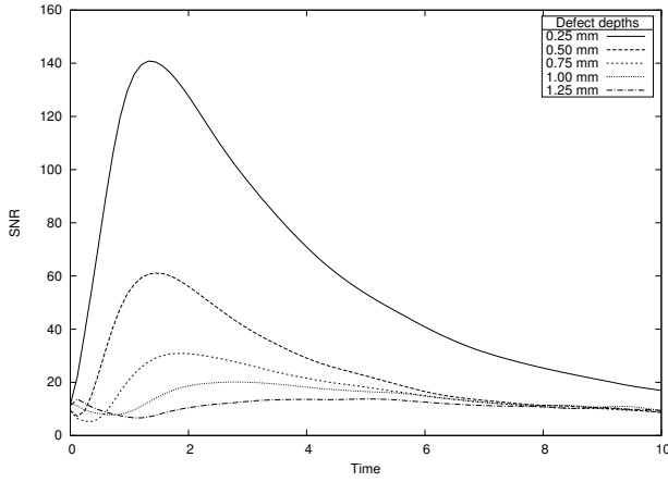
Figure 6: SNR as a function of time for 6 mm diameter defects at depths indicated in this figure.
