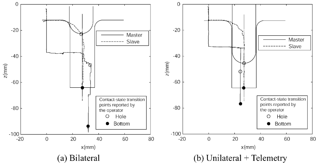
Fig. 18. Arm trajectories during the peg-in-hole task.
