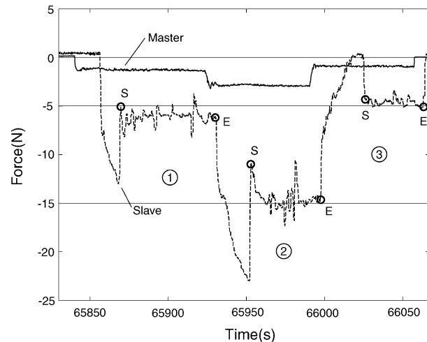
(a) Bilateral
