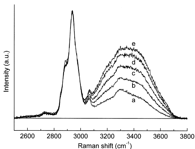
Figure 4. In vivo Raman spectra of the stratum corneum in the spectral interval 2500\text{--}3800\text{ cm}^{-1} . Illustration of the spectral changes due to differences in water content. The spectra were obtained at the thenar, at different depths below the skin surface. Distance to skin surface: (a) 0\text{ }\mu\text{m} ; (b) 75\text{ }\mu\text{m} ; (c) 80\text{ }\mu\text{m} ; (d) 85\text{ }\mu\text{m} ; (e) 90\text{ }\mu\text{m} . The spectra were normalized on the intensity of the protein signal ( 2910\text{--}2965\text{ cm}^{-1} ). Signal collection time for each spectrum, 3 s; excitation wavelength, 730\text{ nm} ; laser power on the skin, 100\text{ mW} .
