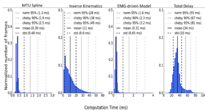
Fig. 7. Computation time on a desktop computer. The histograms (starting from left) respectively depict computation times for the MTU spline, inverse kinematics, and EMG-driven model component as well as the total delay between EMG sampling time and multi-DOF moment computation. The inverse dynamics computation time is not reported as this is constant and does not add substantial latency to the workflow.
