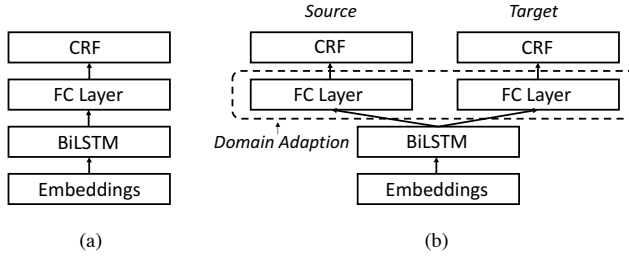
Figure 1: Neural architectures for mention detection and classification. a) Single-task model. b) Multi-task model with domain adoptions.
