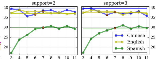
Figure 4: Training with all data (Run 1) vs early stopping on the example of joint-model ensembles with different minimal support. Subtype+Realis test set F1-score for the ensembles after each training epoch (thick); the score after the last estimated training epoch (orange diamond); the same ensemble trained with early stopping (thin).
