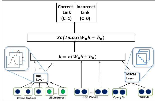
Figure 2: Architecture of our neural EL system. The input to the system are: a document D containing the query mention m and the corresponding Wikipedia candidate link l_i \in L , where L is the set of all possible links extracted from the fast match step.
