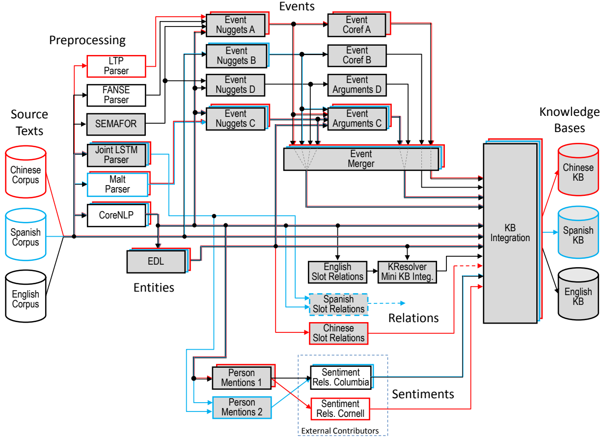
Figure 1: System architecture
