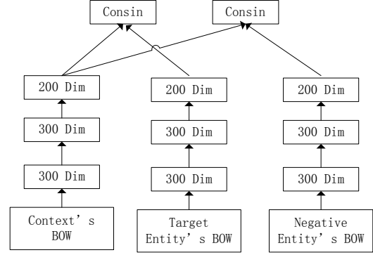
Figure 4: The architecture of DSSM
