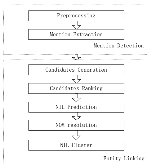
Figure 1: The architecture of TAI’s system
