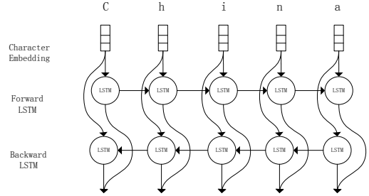
Figure 3: The architecture of character embedding
