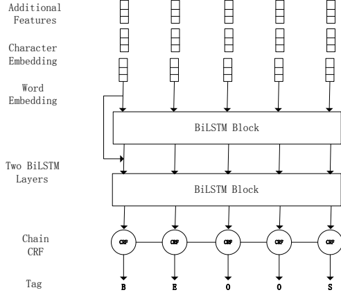
Figure 2: The architecture of Mention Extraction
