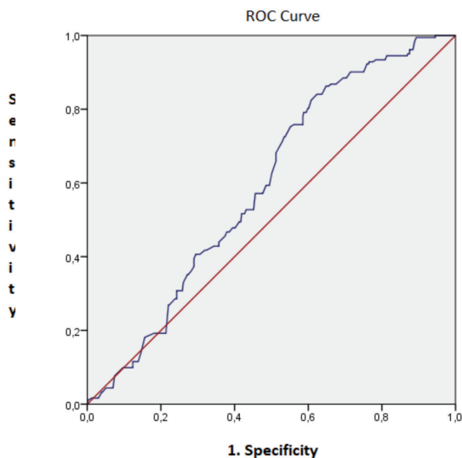
Figure 1. ROC analysis
