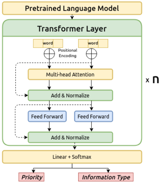
Figure 3: Detailed model for multitask event detection [4, 6].
