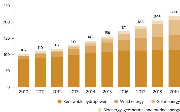
Installed renewable energy-generating capacity in developing countries, by technology, between 2010 and 2019 (watts per capita)
