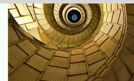
Hyperbolic spirals in a spiral staircase
