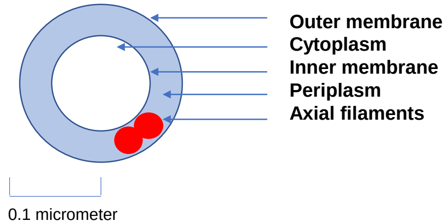
Fig. 1 Sectional view of a spirochete cell
