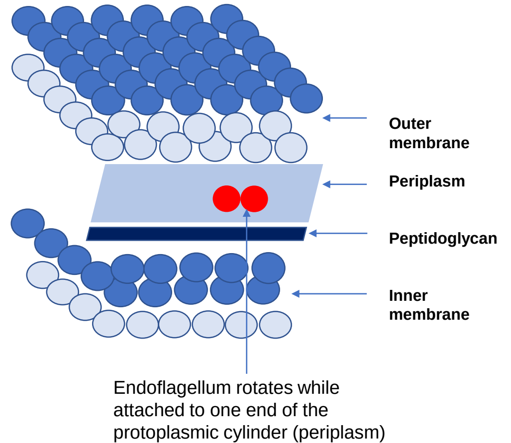
Fig. 3 Endoflagellum motion in periplasm
