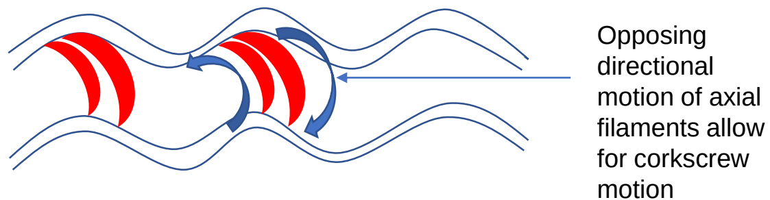
Fig. 2 Axial filament mechanics
