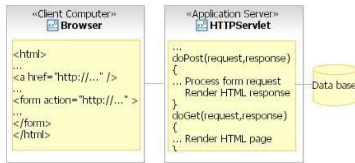
Abb. 5: Figure 3: Servlet Execution
