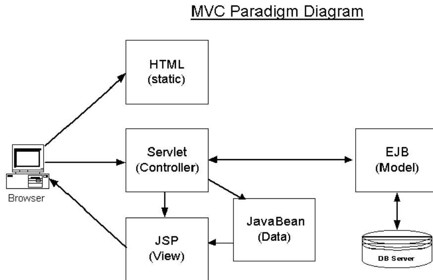
Abb. 8: Figure 6: MVC Execution
