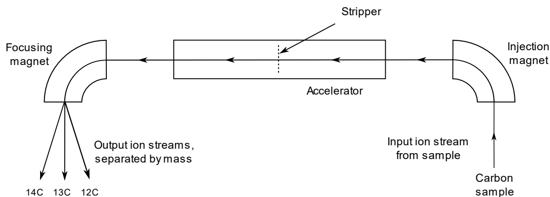
Figure 5 | Simplified schematic layout of an accelerator mass spectrometer used for counting carbon isotopes for carbon dating
