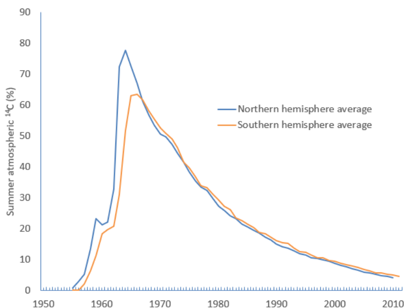
Figure 2 | Atmospheric ^{14}\text{C} for the northern and southern hemispheres, showing percentage excess above pre-bomb levels. The Partial Test Ban Treaty went into effect on 10 October 1963. [38]
