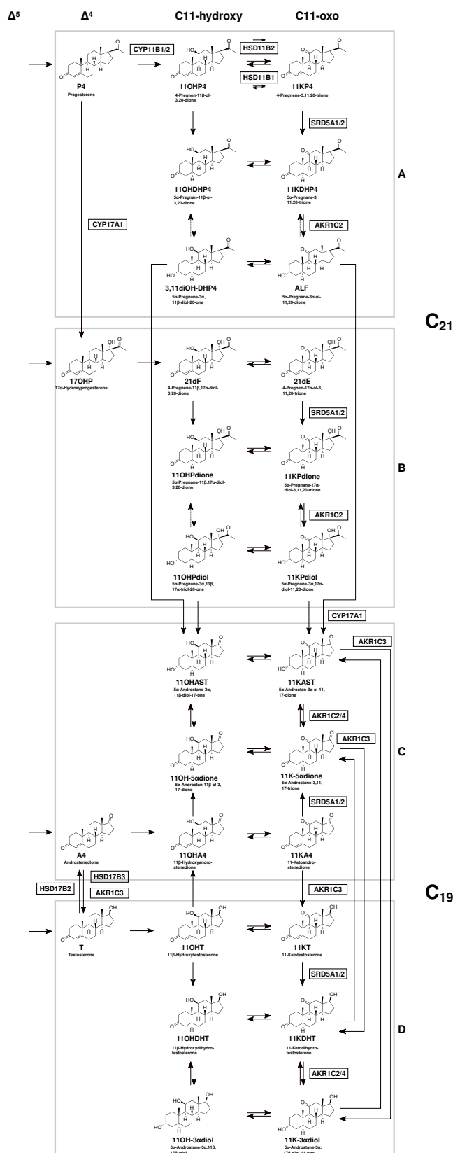
Figure 3 Abbreviated routes to 11-oxygenated androgens with transformations (black arrow) annotated with the HGNC symbol (boxed text) of the gene for the enzyme that catalyzes the transformation. The four groups of steroids are distinguished by the C17 substituent configuration associated with four distinct precursors, A: the conversion of progesterone B: the conversion of 17-hydroxyprogesterone by CYP11B1, SRD5A, and AKR1C2 in the C11-hydroxy and -oxo C 21 steroids C: the conversion of androstenedione D: the conversion of testosterone by CYP11B1, HSD11B, SRD5A, AKR1C3 and AKR1C2/4 in the C11-hydroxy and -oxo C 19 steroids. CYP17A1 catalyzes the C 21 steroids to C 19 steroids. Some transformations which are presumed to exist but not yet shown to exist are depicted with dotted arrows. Some CYP17A1 mediated reactions that transform 11-oxygenated androgens classes (grey box) are omitted for clarity. \Delta^5 compounds that are transformed to \Delta^4 compounds are also omitted for clarity.
