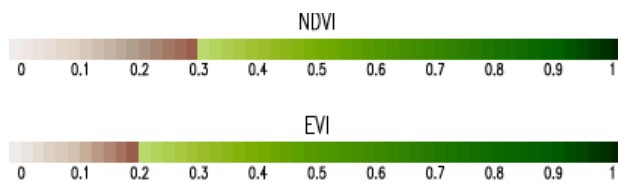
Figure 7: MODIS VI Color Palettes for NDVI (upper) and EVI (lower) products as used in this document.
