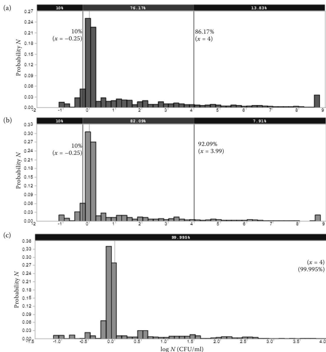
Figure 1. The probability distribution of B. cereus at the time of pasteurised milk consumption (a) general case, (b) UBD+1 case, and (c) idealised case
