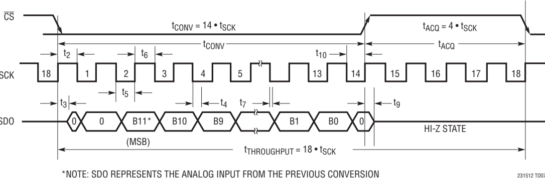
Figure 7: LTC2315-12 Serial Interface Timing Diagram (SCK Continuous)
