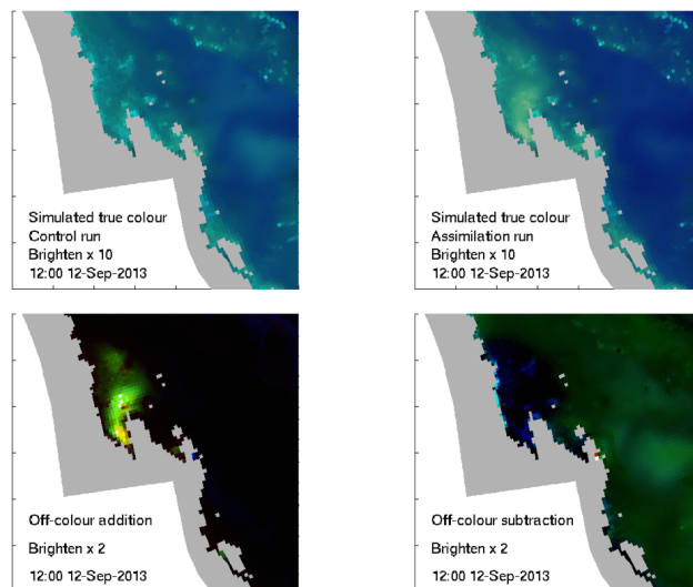
Figure 17. The simulated true-colour image on 12 September 2013 of the control run (top left) and EXP4 assimilation run (top right). The difference between the remote-sensing reflectance in the control and assimilated runs was used to quantify the colour (referred to as off-colour) added (i.e. greater surface expression, bottom left) and subtracted (i.e. less surface expression, bottom right) due to the updating of optically active constituents in the assimilation run (see Fig. 16 for more details). Note that the off-colour images have a smaller brightening factor as the MODIS true-colour stretch saturates the features that are of most interest. Simulated true-colour images are not falsely coloured, and thus do not require a colour map, nor are they 2-D as they have a depth of field, being based on reflectance from multiple depths and the bottom (Baird et al., 2016a). Thus simulated true colour can be considered a photograph of the optical state of the different model runs and, like observed true colour, a powerful and intuitive visualisation tool for water clarity in BGC models.
