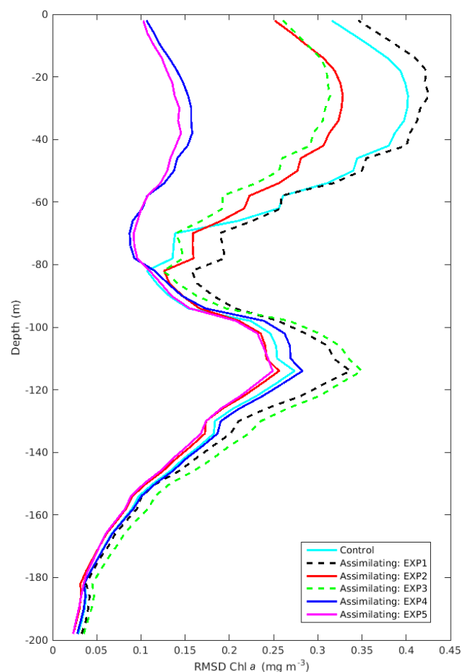
Figure 9. A profile of the temporal mean Chl a RMSD between the glider observations presented in Fig. 7 and the non-assimilating control (cyan), EXP1 (black dashed; note that the mean RMSD is calculated using a short time period), EXP2 (red), EXP3 (green dashed; note that the mean RMSD is calculated using a shorter time period), EXP4 (blue) and EXP5 (magenta).
