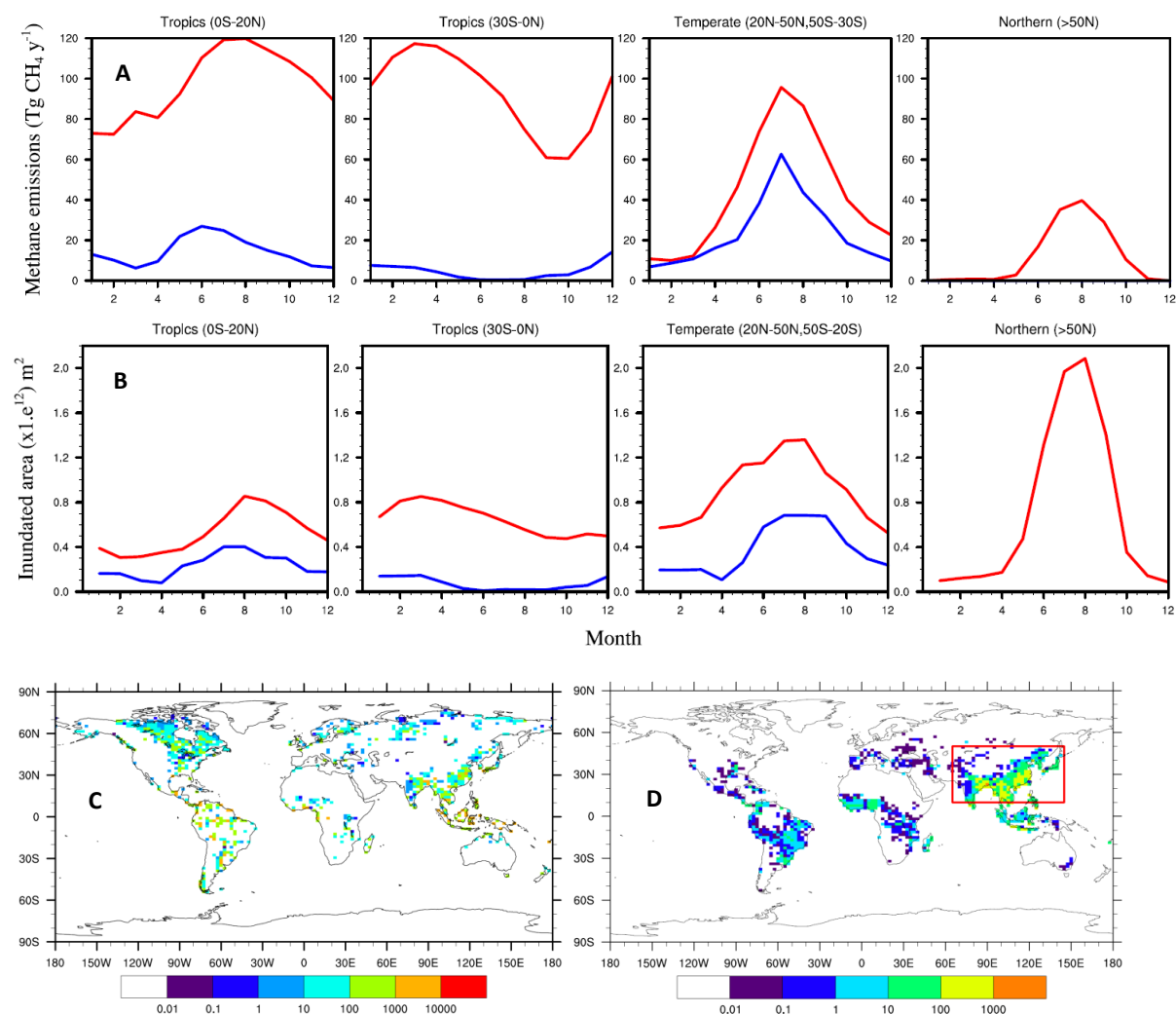
Fig. 14. Seasonal variation of methane emissions ( A ) and inundated areas ( B ) in the four defined regions for natural wetlands (red) and rice paddies (blue). ( C ): The global distribution of the mean methane emission rates (units: \text{mg CH}_4 \text{ m}^{-2} \text{ d}^{-1} ) during the period 1993–2004 from natural wetlands. ( D ): The global distribution of annual averaged methane emissions (units: \text{mg CH}_4 \text{ m}^{-2} \text{ d}^{-1} ) for the year 2000 from rice paddies. (Asian monsoon regions are in red box).
