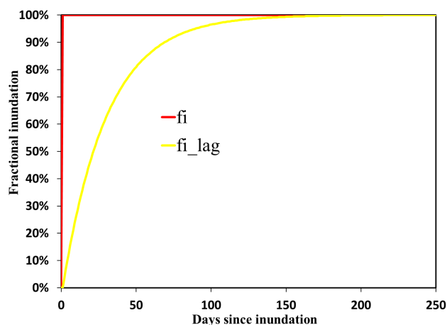
Fig. 2. An illustrative diagram of the impact of redox potential on inundated fraction. f_i is representative of the inundated fraction that is predicted by the model. f_{i\text{lag}} is the inundated fraction that is actively producing methane.
