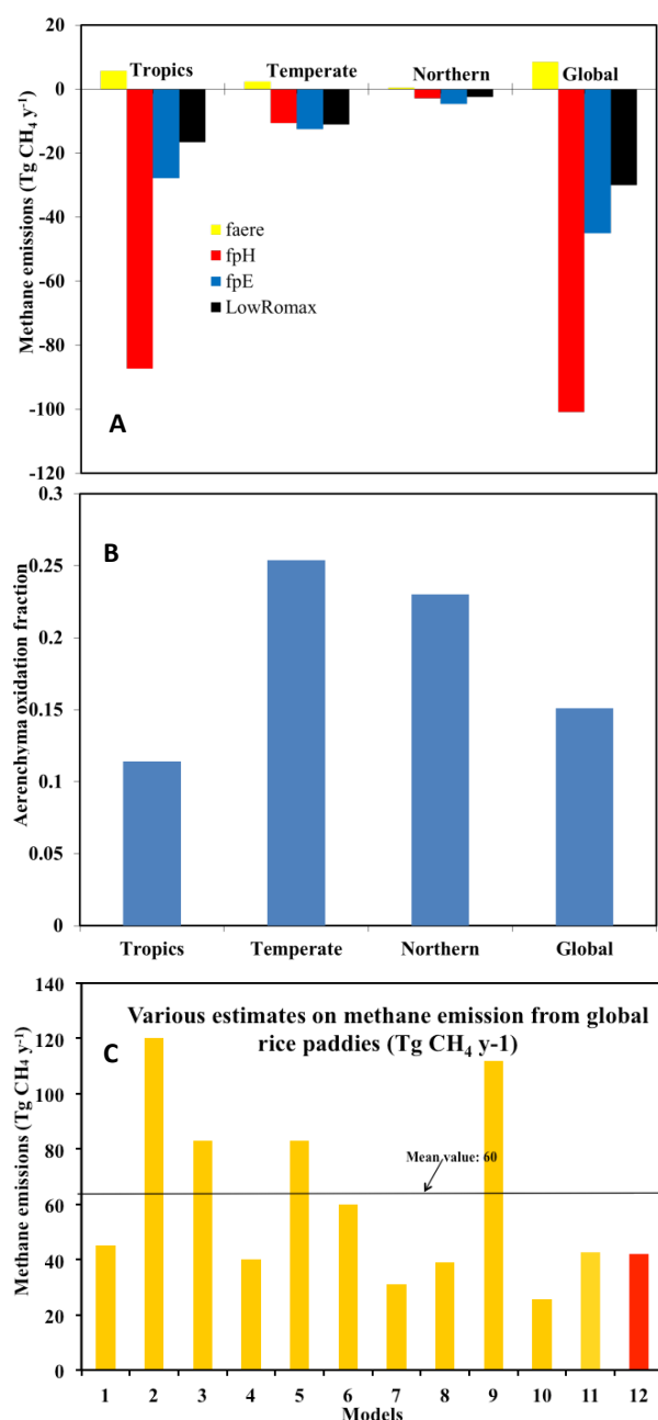
Fig. 13. A: Sensitivity analysis of each variable. The number on the y-axis indicates the change in net annual mean methane emission associated with changes in each variable. B: Prognostic aerenchyma oxidation fractions at different regions. C: Comparison of global methane budget from rice paddies estimated in our model and other models. 1: Seiler et al. (1984); 2: Holzapfel-Pschorn and Seiler (1986); 3: Bouwman (1990); 4: Sass (1994); 5: Hein et al. (1997); 6: Wuebbles and Hayhoe (2000); 7: Scheehle et al. (2002); 8: Olivier et al. (2005); 9: Chen and Prinn (2006); 10: Yan et al. (2009); 11: Spahni et al. (2011); 12: this model (red).
