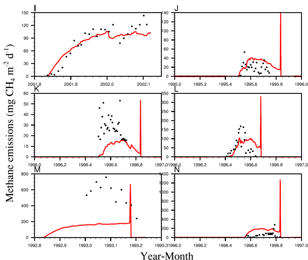
Fig. 10b. (continued). I: Central Java, Indonesia; J: New Delhi, India, 1995; K: New Delhi, India, 1996; L: Beijing, China; M: Lampung, Indonesia; N: Cuttack, Indonesia. Please see Table 1 for site descriptions.
