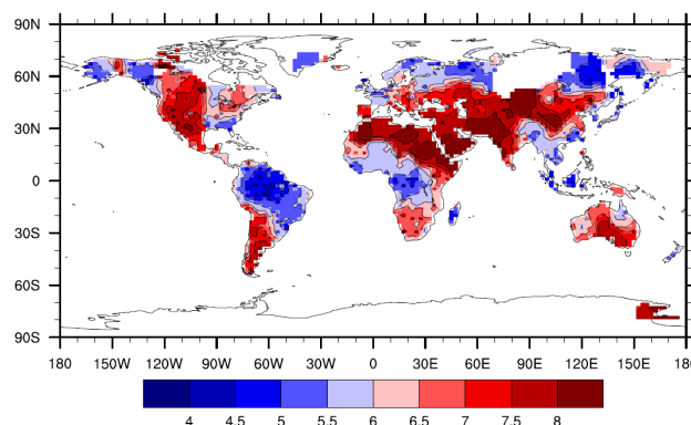
Fig. 5. The global distribution of soil pH. Data Sources: IGBP-DIS (see Tempel et al. (1966) and Pleijsters (1986)).
