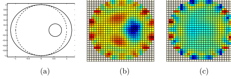
FIGURE 3. Effect of a boundary geometry error. (a) The ellipse with solid line was the true imaging domain and the circle in dashed line was the computational model domain. The small disk inside the domain was an anomaly. Complex conductivity values of the anomaly and the background were those of the banana and the saline, respectively. (b) and (c) are reconstructed static images (real-part images) at frequencies \frac{\omega_1}{2\pi} = 100 Hz and \frac{\omega_2}{2\pi} = 50 kHz, respectively. Each image was reconstructed using the boundary voltage data from the homogeneous computational model domain as the reference data. This figure is quoted from [31].
