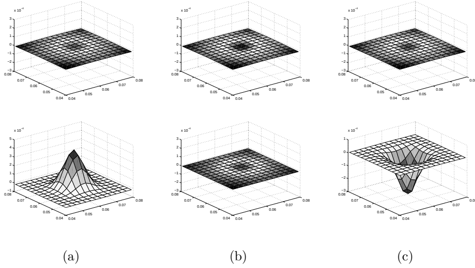
FIGURE 7. Frequency-difference trans-admittance map: real and imaginary parts of g_2 - \alpha g_1 with three different values cases; (a) \mu = \left(\frac{\epsilon_{2,c}}{\epsilon_{2,n}} - \frac{\sigma_c}{\sigma_n}\right) > 0 (b) \mu = 0 (c) \mu < 0 . We quote this figure from [19].
