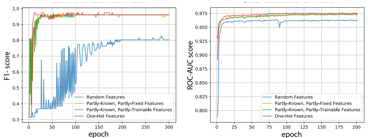
(a) Features' Impact on Node-Classification Task
