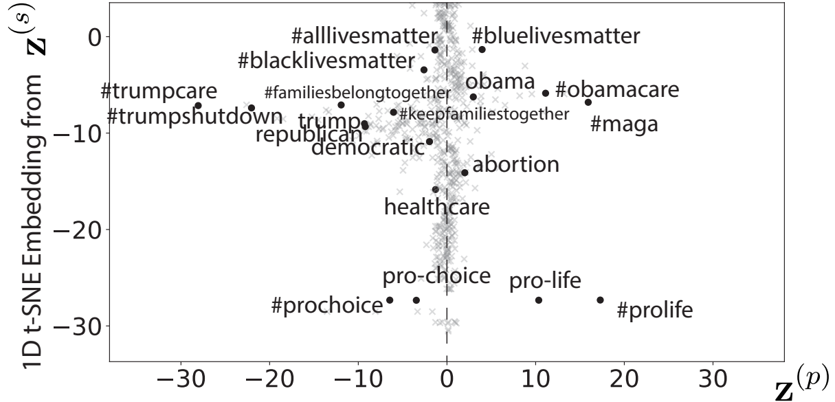
Figure 3.3: Visualization of the political polarities in our embedding results. The horizontal axis gives the values of the polarity score \mathbf{z}^{(p)} , and the vertical axis is a 1D t-SNE value (which we use to facilitate visualization) that we calculate from the semantic embedding \mathbf{z}^{(s)} .
