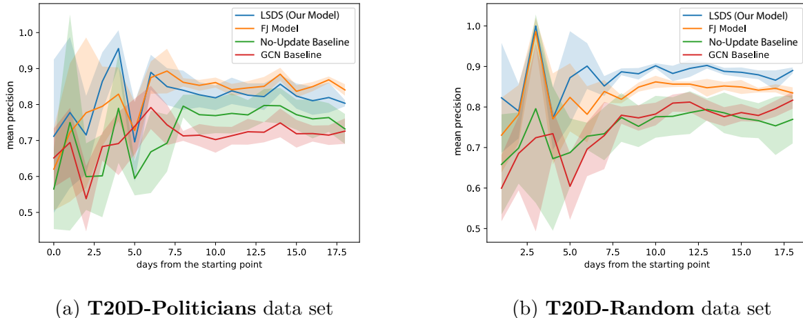
Figure 4.5: The mean precisions (i.e., PR-AUCs) of the predictions of temporal interactions after different numbers of days. The solid curves indicate the mean values, and the filled areas indicate the standard deviations.
