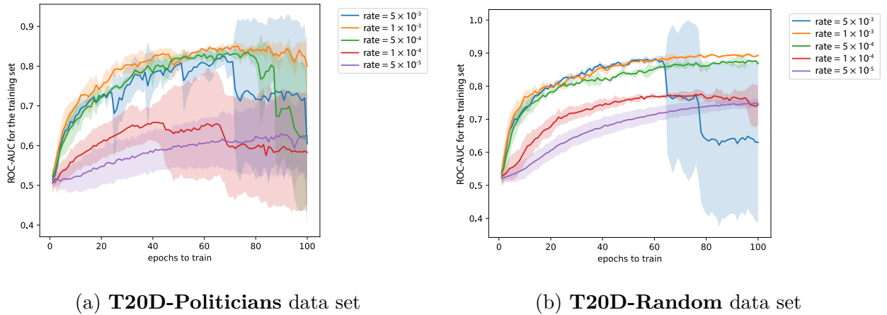
Figure 4.9: The ROC-AUCs of our LSDS model for the training set after each epoch for various learning rates. We observe similar trends for the testing set. Larger loss values indicate worse performance.
