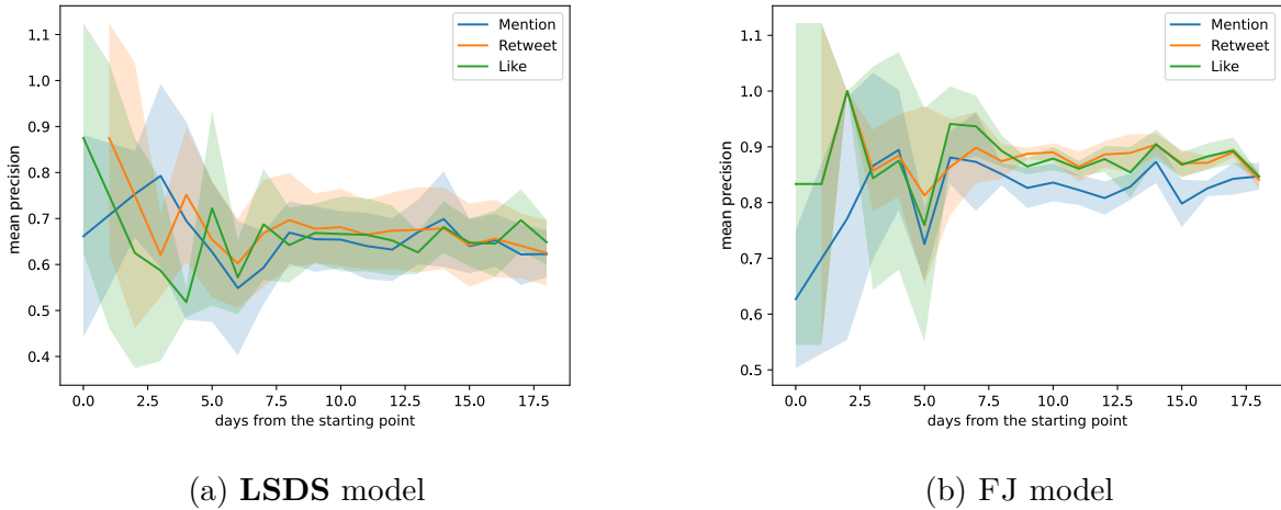
Figure 4.6: The mean precisions (i.e. PR-AUCs) of the predictions of different types of temporal interactions in the T20D-Politicians data set after different numbers of days. The solid curves indicate the mean values, and the filled areas indicate the standard deviations.
